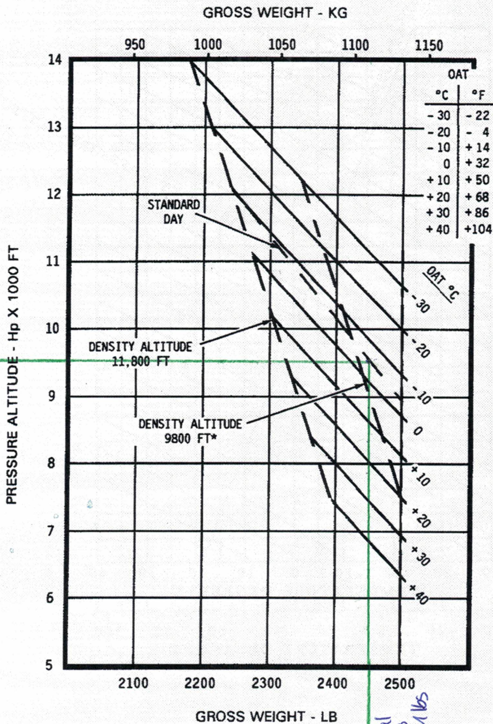
IGE HOVER CEILING VS. GROSS WEIGHT
