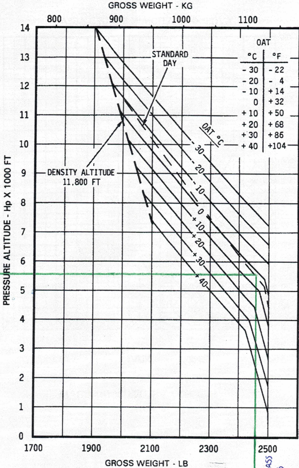
OGE HOVER CEILING VS. GROSS WEIGHT
