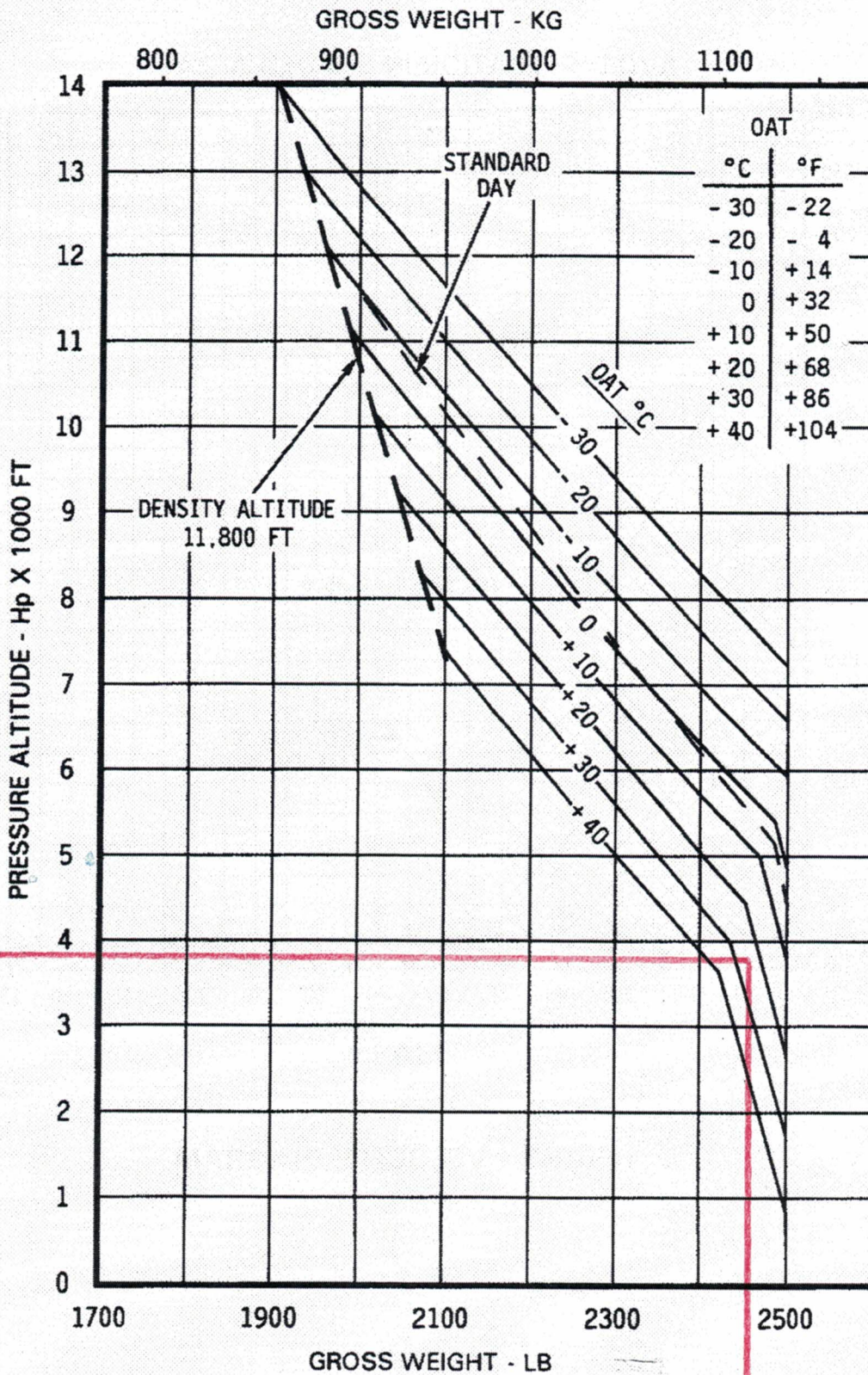
OGE HOVER CEILING VS. GROSS WEIGHT
